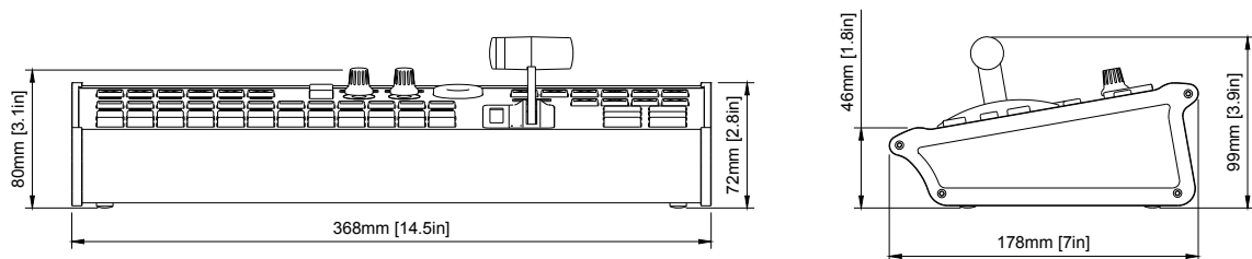
Figure 1: Technical drawing of Air Fly Pro with key dimensions and layout details.
